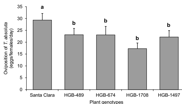
Fig. 5 Oviposition of T. absoluta on five tomato genotypes. Bars show the average number of eggs laid (+SE) by T. absoluta mated females on single leaflets from five different tomato genotypes in a no-choice test. The susceptible genotypes are Santa Clara variety and HGB-489, and the resistant genotypes are HGB-674, HGB-1708, and HGB-1497. Different letters denote significant differences (GLM with contrast, P \leq 0.05 ) among plant genotypes
