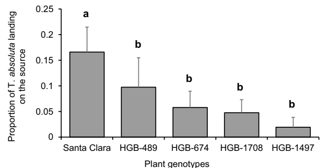
Fig. 3 Behavioral response of T. absoluta toward tomato plants in a wind tunnel on the first hour of the scotophase (size 3 \times 1 \times 1 \text{ m}^3 , wind speed 0.35 \text{ m/s} , 23 \pm 2^\circ\text{C} , and 70 \pm 5\% \text{ RH} ). Bars show mean proportion ( \pm \text{SE} ) of T. absoluta mated females that landed on each of the five tomato genotypes in a no-choice test. Leaves from each tomato genotype were placed at the end of the wind tunnel, and one female was placed in a platform on the opposite site. The susceptible tomato genotypes are Santa Clara variety and HGB-489 and the resistant genotypes are HGB-674, HGB-1708, and HGB-1497. Different letters denote significant differences (GLM with contrast, P \leq 0.05 ) among plant genotypes
