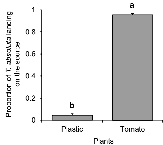
Fig. 2 Flight response of T. absoluta toward tomato and plastic plants in a wind tunnel on the first hour of the scotophase (size 63 \times 63 \times 200 \text{ cm}^3 , wind speed 0.25 \text{ m/s} , 23 \pm 2^\circ\text{C} , and 70 \pm 5\% \text{ RH} ). Leaves from the tomato genotype Santa Clara variety were placed simultaneously with green plastic leaves at one end of wind tunnel, and one T. absoluta mated female was placed in a platform on the other end. Bars show mean proportion ( \pm \text{SE} ) of T. absoluta mated females that landed on each of the two plants in a choice test. Different letters denote significant differences (GLM P \leq 0.05 ) among plants
